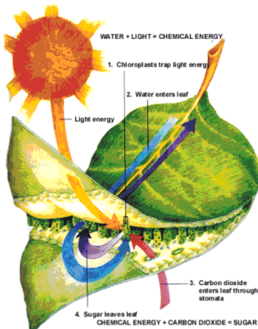
Figure 3.1 Photosynthesis 6
